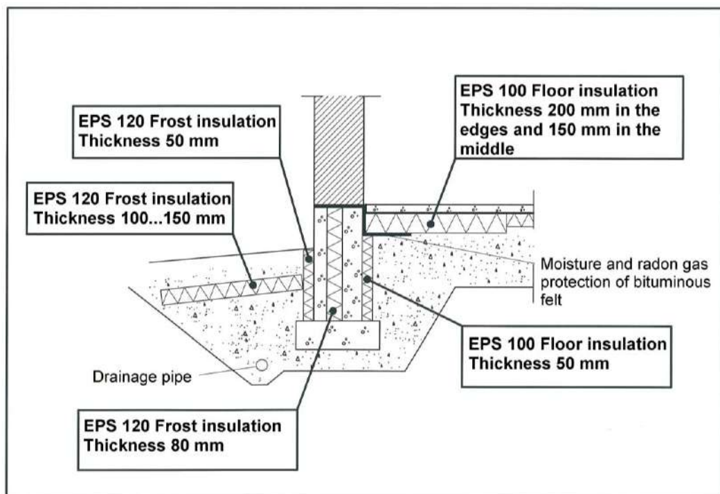
Figure 16: Example of how to use EPS frost and floor insulation materials in ground slab structures.
