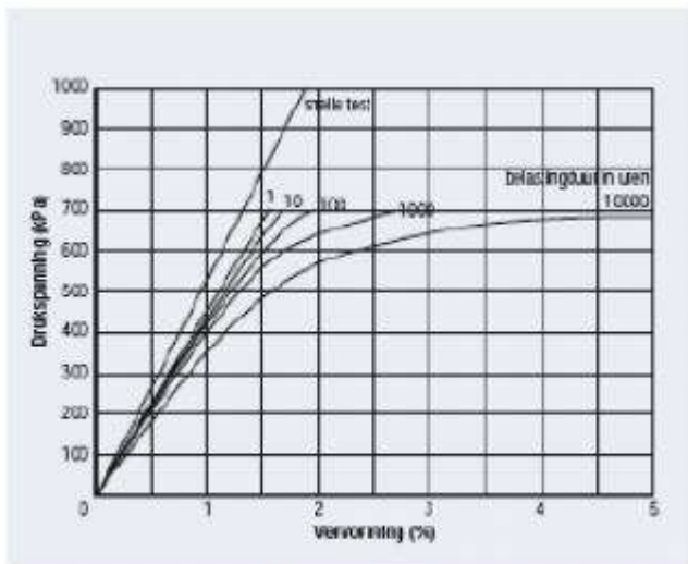
Figure 5: Spanning/verormingsrelatie in belastingniveau
